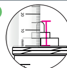
Measure the pin length of the valve when it is in the open position. (must measure between 13-16mm)
